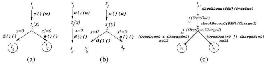
Fig. 5. (a) Component STS (b) Goal STSs STS_g & STS_{g'} (c) STS for NewChecker
