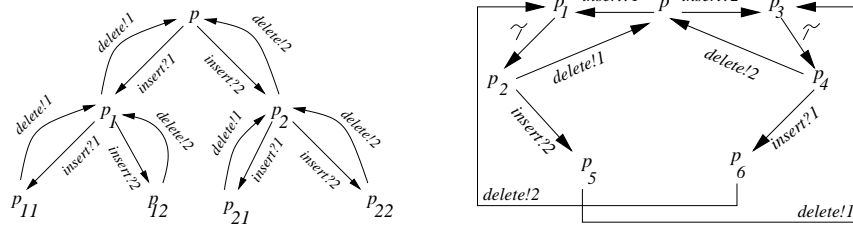
Fig. 2. a. stack (2, 2) b. multi_link_buffer (2, 2)
