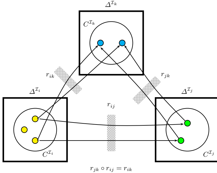
Fig. 5. Compositionally Consistent Domain Relation
