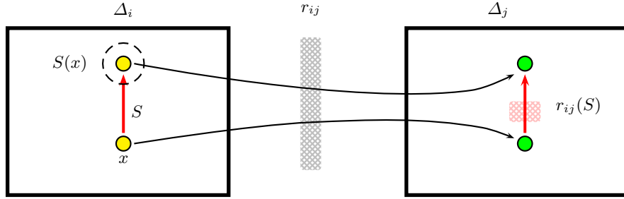
Fig. 3. Successor Set and Role Image
