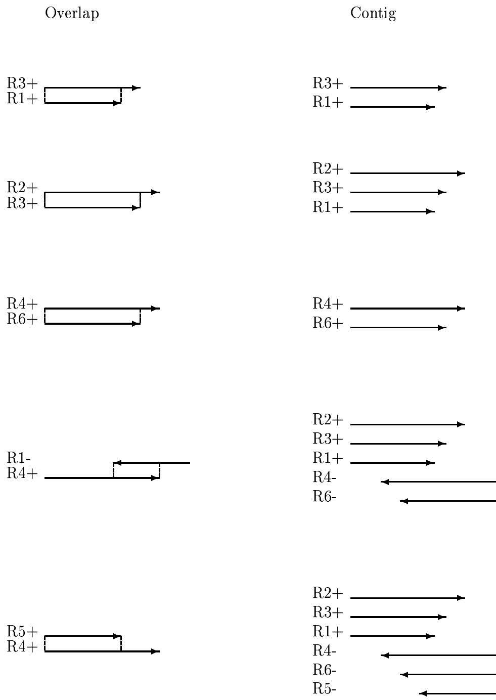
Figure 2.5 The current overlap and the resulting contig
